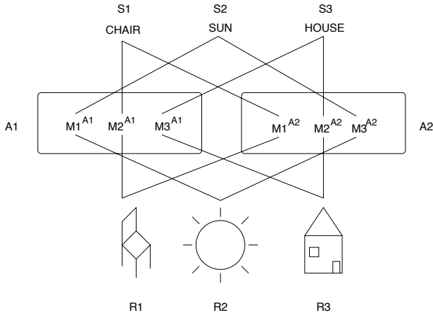
Figure 1. Illustration of the model for communication development. The figure shows three physical objects that function as referents (R1...R3). Both agents A1 and A2 have a conceptual system that maps these external referents to internal meanings (M1...M3 for each agent). The aim is to form a mapping between meanings and words (S1...S3) so that information about objects or situations in the environment can be shared.
